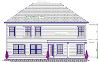
BACK ELEVATION
